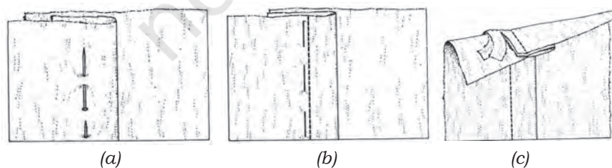
Fig. 3.21 (a, b, c) Tucked seam
